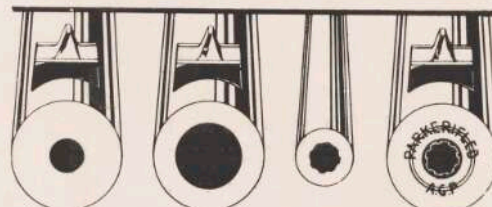
THE ORIGINAL BARREL, NO LONGER ACCURATE BORED OUT TO RECEIVE THE PARKER RIFLED TUBE WHICH IS INSERTED, MAKING A SUPER ACCURATE RIFLE
